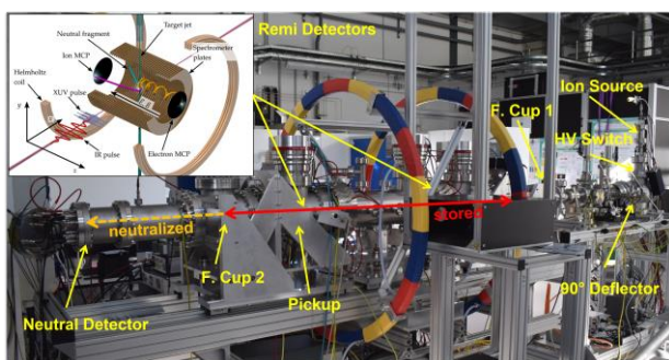
Figure 1. Image of the TrapREMI setup. A EIBT beam-transport line follows the ion source. The REMI comprises several spectrometer electrodes, three detector modules, and a pair of Helmholtz coils, see inset. In the TrapREMI, the ion beam is brought to interact with IR laser pulses or a neutral jet. The overall setup is about 5 m long and 2 m in height.
