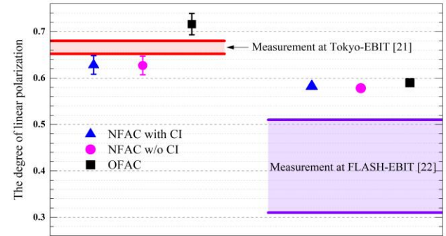
Figure 1. Measurements (Bi ions at 51.1 keV [1] and Kr ions at 8.76 keV [2]) and theoretical calculations of L-RR x-ray linear polarizations. The blue triangles and pink circles represent the calculations of NFAC with and without CI, respectively. The black squares represent the calculations of the OFAC which are reported in previous papers.
