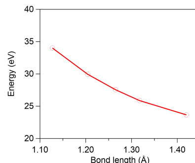
Figure 3. The calculated potential energy curve of Auger final state.
