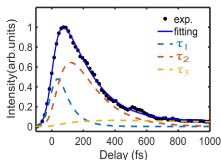
Figure 1. The decay profile of the photoelectron intensity integrated over all possible excited-states.
